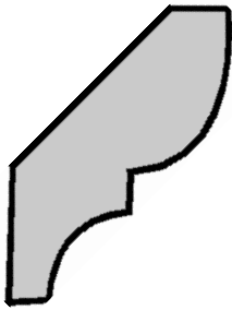
#74 2" Bedmould 9/16" x 1 3/4" 1 7/16" Rise 1 1/8" Projection
