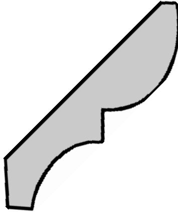
#70 3" Bedmould 5/8" x 2 3/4" 2 5/16" Rise 1 5/8" Projection
