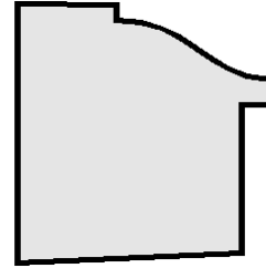
#8808 1 1/4" x 1 7/32" Rabbet: 1/2"
